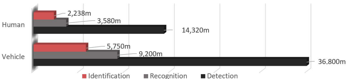
DRI Ranges (Using Johnson's Criteria)
